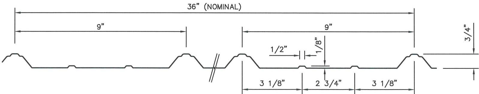
PANEL PROFILE
